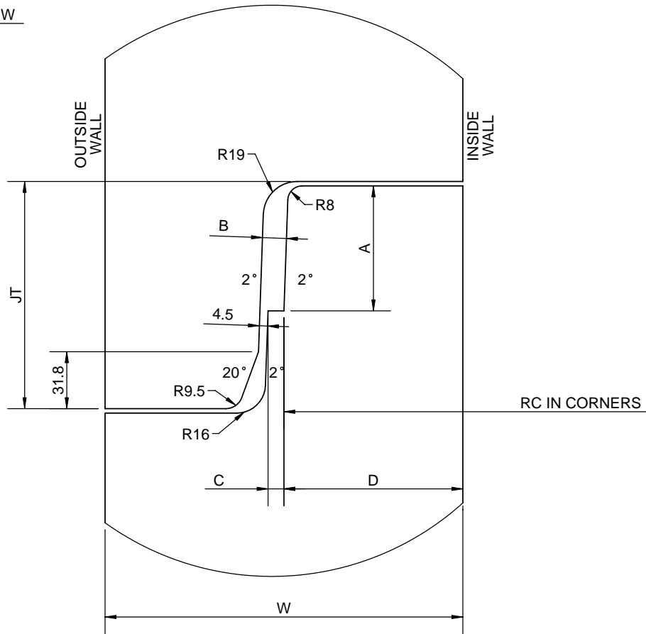
JOINT DETAIL
